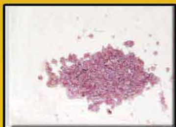
Purple color indicates non-acidic
