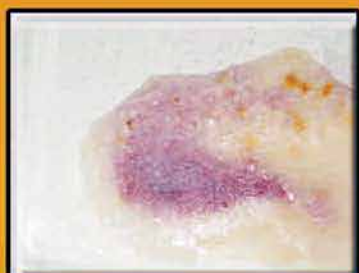
Foaming indicates neutralization in process
