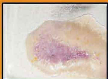
Neutralizing sulfuric acid
